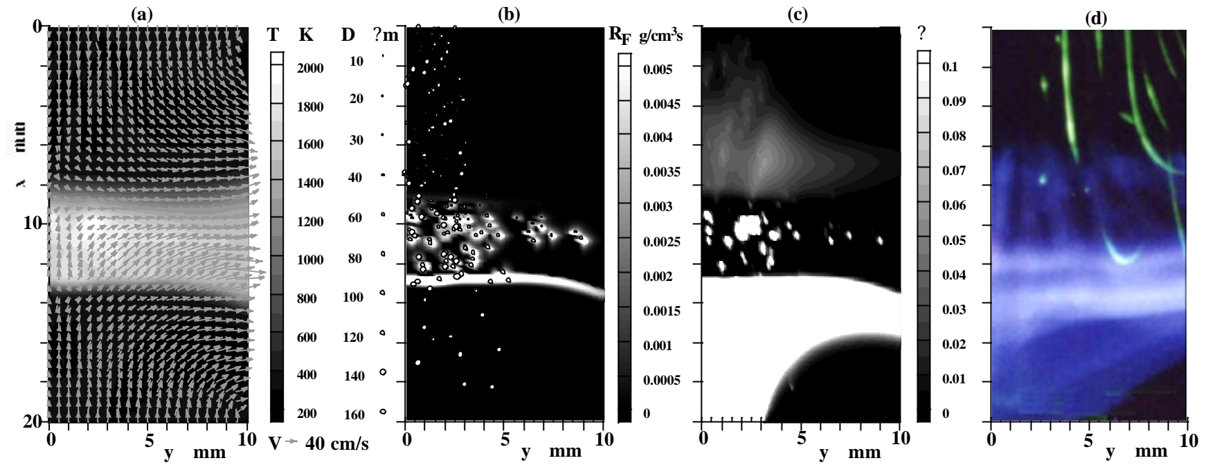
Fig. 4 Numerical results ( t = 25 ms after spray injection) and the corresponding flame photograph
