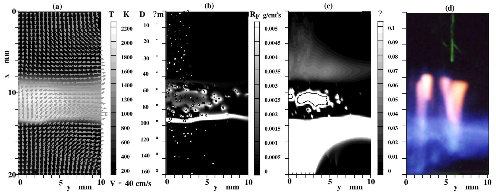
Fig. 5 Numerical results ( t = 30 ms after spray injection) and the corresponding flame photograph
