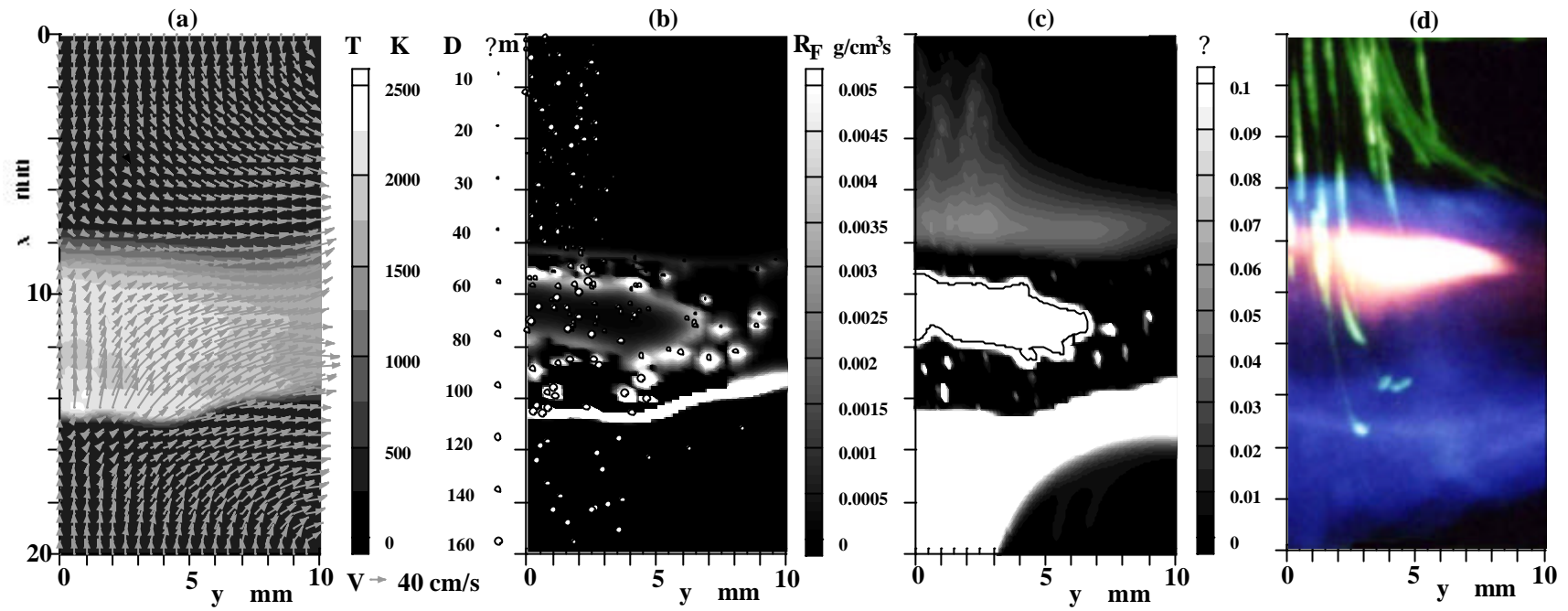
Fig. 6 Numerical results ( t = 35 ms after spray injection) and the corresponding flame photograph
