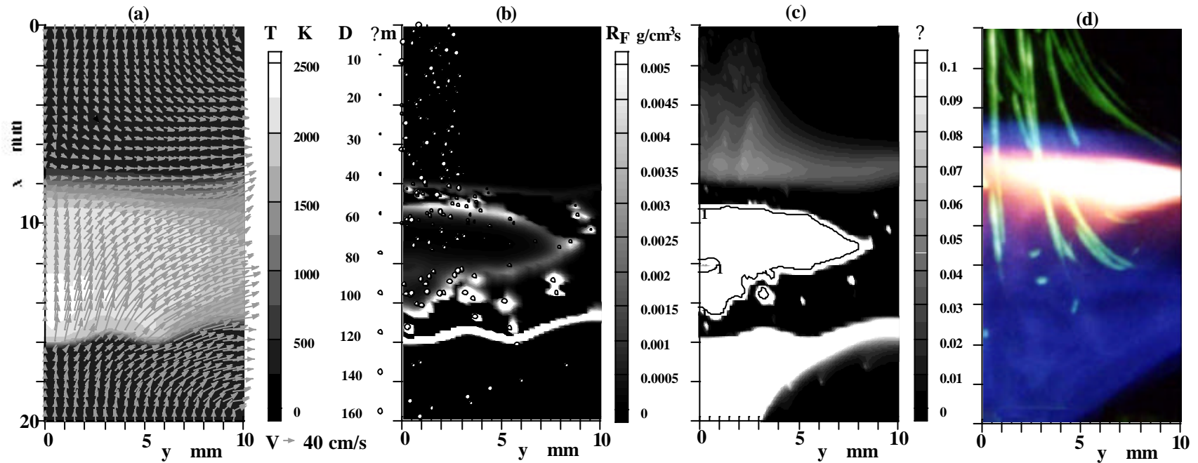
Fig. 7 Numerical results ( t = 40 ms after spray injection) and the corresponding flame photograph
